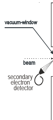
Fig. 7 Hit detection by detecting the secondary electrons emitted from the vacuum window when an ion passes.
