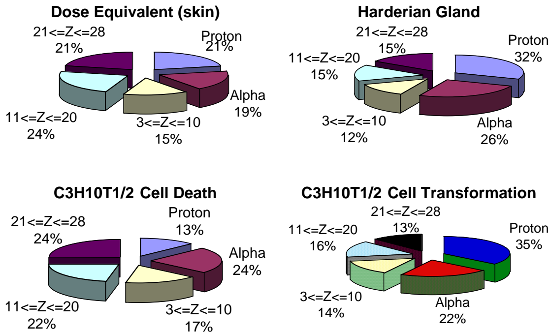
Figure G. 1. Primaries and Secondaries Inside 5 g/cm 2 of Aluminum
